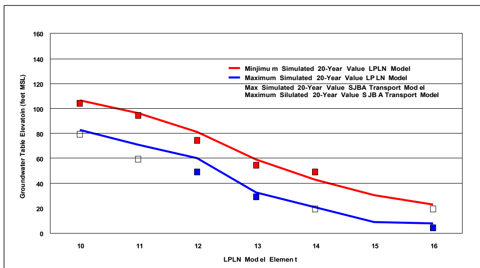
Figure 6-6 Simulated Groundwater Table Elevations, 2000-2020 - San Juan Creek Arm
