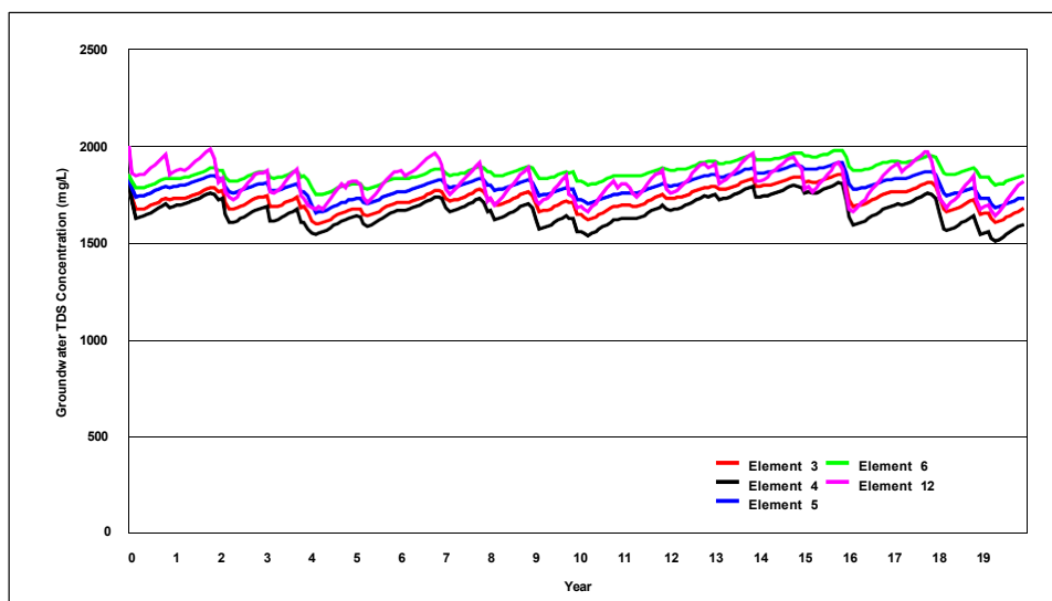
Figure 6-9 Simulated Groundwater TDS Concentrations – Oso/Trabuco Creek Arm
