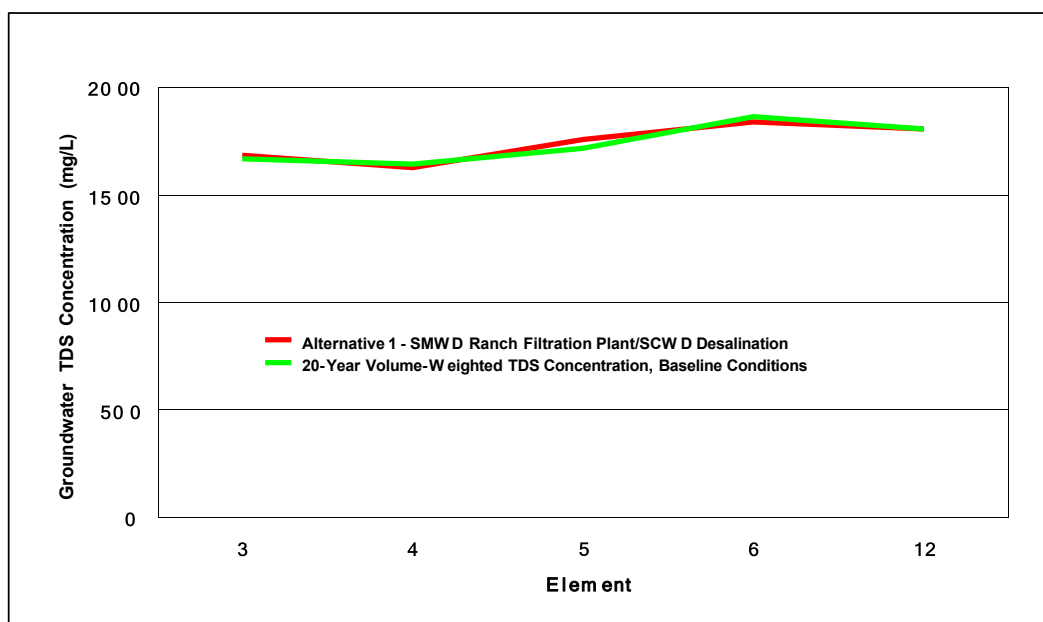
Figure 6-16 Comparison of Baseline Conditions with Management Alternative 1 – Oso/Trabuco Creek Arm)
