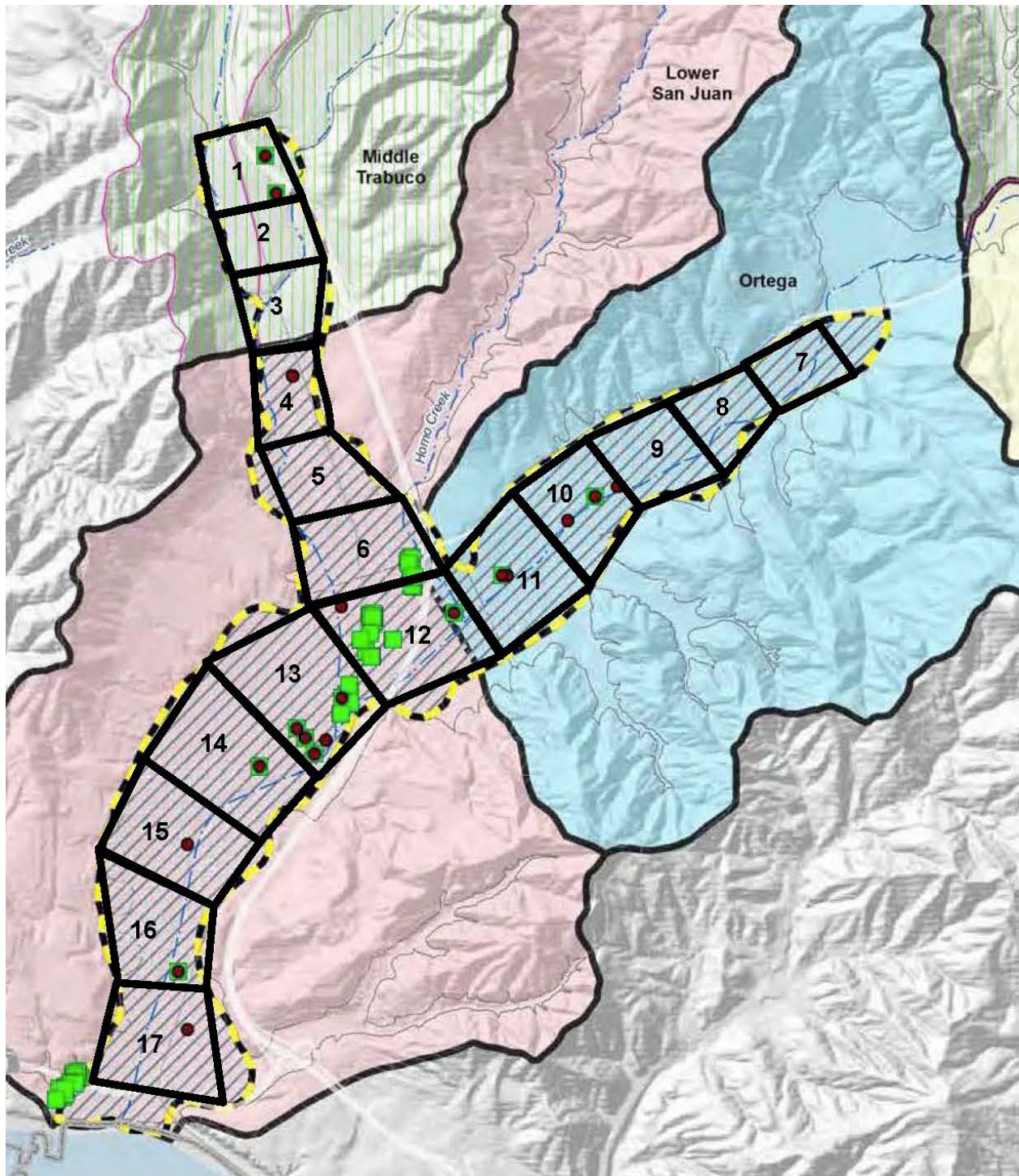
Figure 6-1 Elements of the Lower Basin LPLN Model
