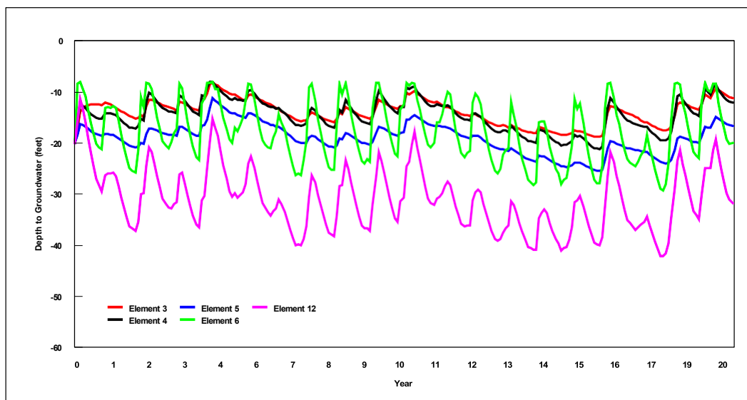
Figure 6-5 Simulated Depth-to-Groundwater under Baseline Conditions – Oso/Trabuco Creek Arm
