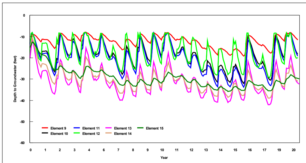
Figure 6-4 Simulated Depth-to-Groundwater under Baseline Conditions - San Juan Creek Arm
