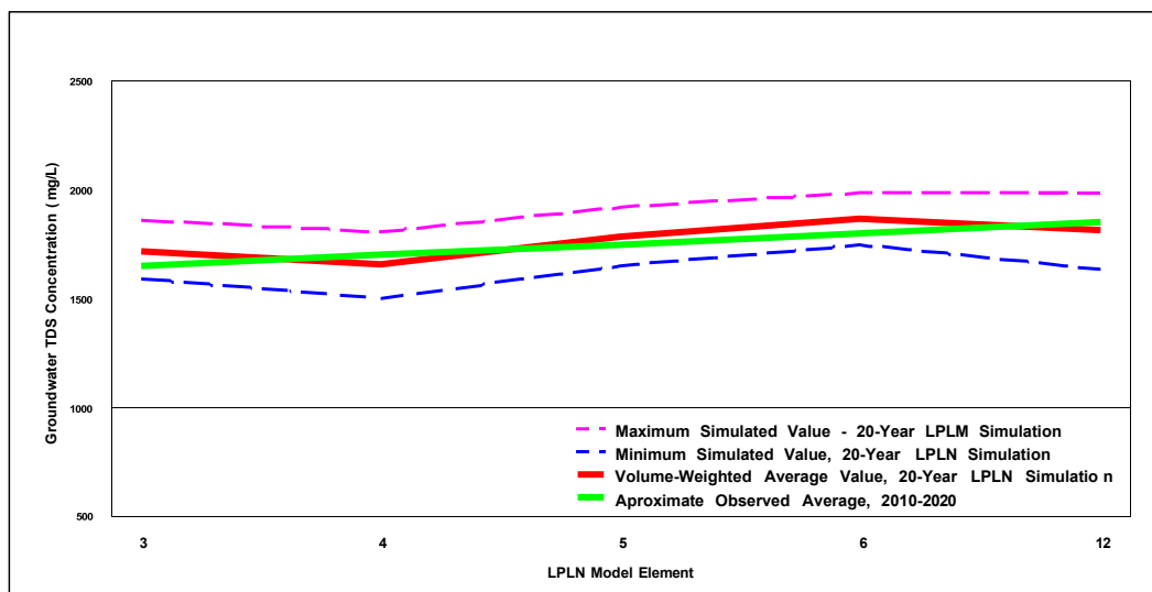
Figure 6-11 Simulated vs. Observed Groundwater TDS Concentrations in the 2000s– Oso/Trabuco Creek Arm
