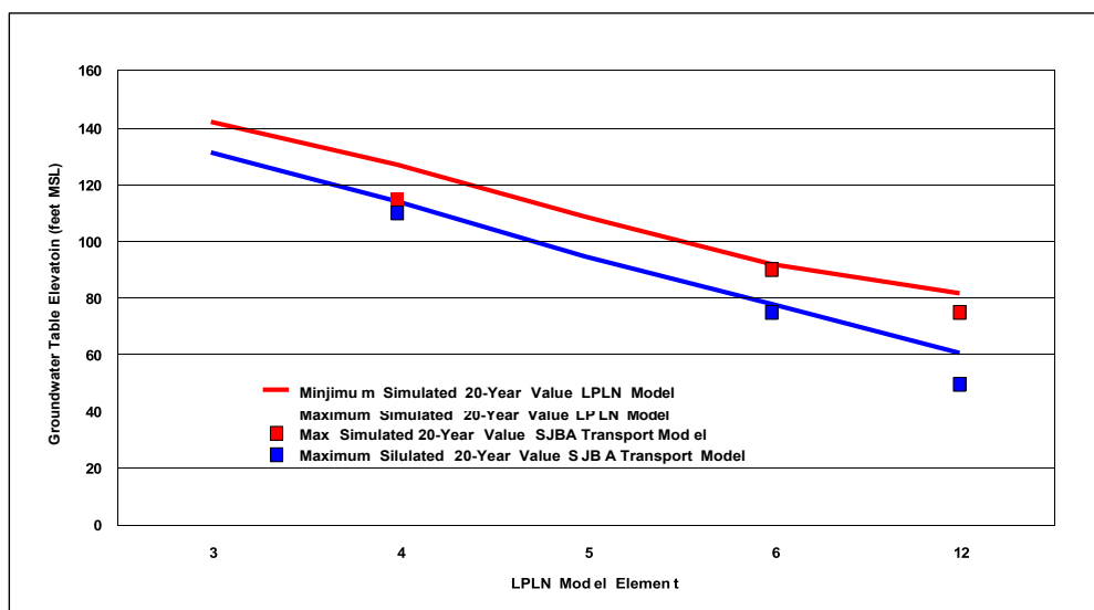
Figure 6-7 Simulated Groundwater Table Elevations, 2000-2020 – Oso/Trabuco Creek Arm
