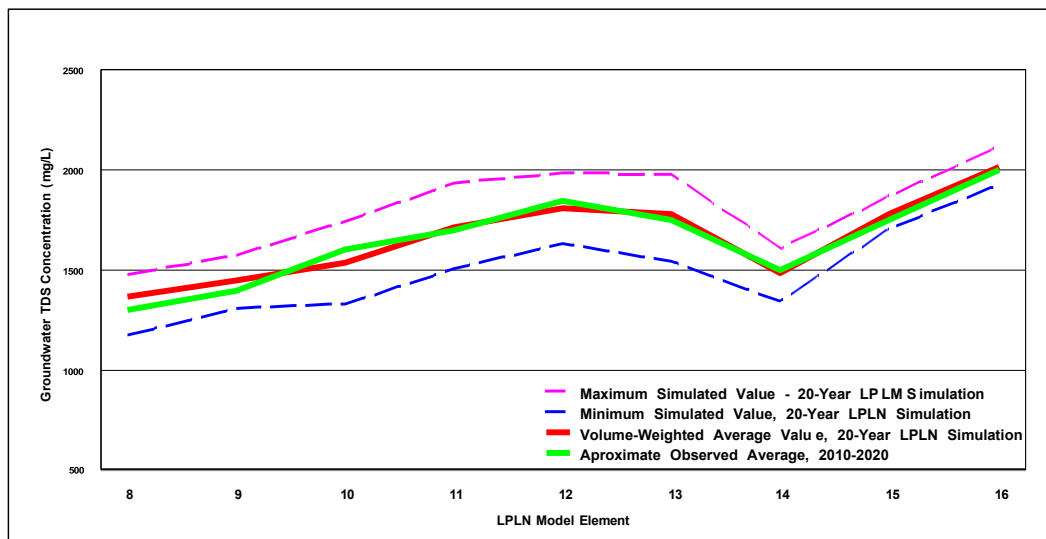
Figure 6-10 Simulated vs. Observed Groundwater TDS Concentrations in the 2000s– San Juan Creek Arm
