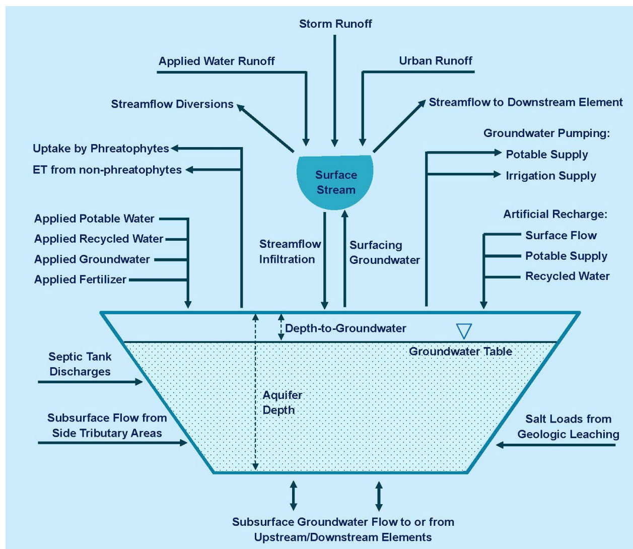
Figure 6-2 LPLN Element Schematic – Ground and Surface Water Components of Each Model Element
