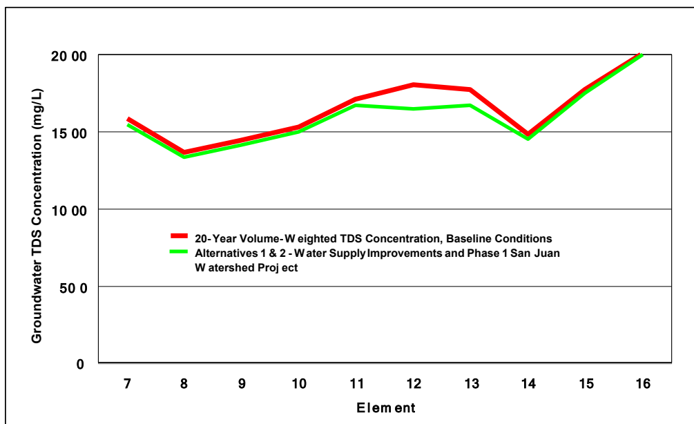
Figure 6-17 Comparison of Baseline Conditions with Management Alternatives 1 and 2 – San Juan Creek Arm
