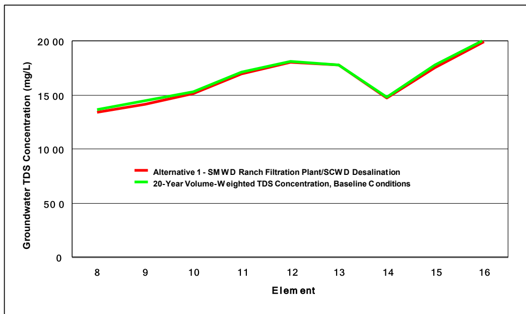
Figure 6-15 Comparison of Baseline Conditions with Management Alternative 1 – San Juan Creek Arm
