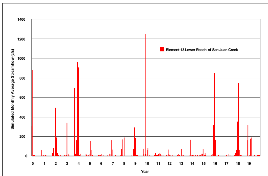
Figure 6-14 Simulated Streamflow at Element 13 (Downstream Reach of San Juan Creek)
