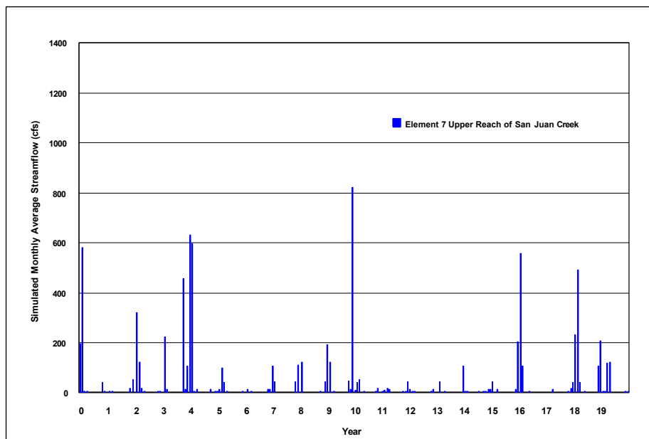
Figure 6-13 Simulated Streamflow at Element 7 (Upstream Reach of San Juan Creek)
