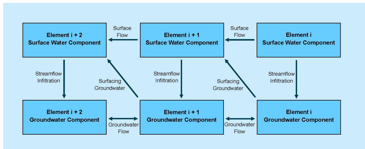
Figure 6-3 Schematic of LPLN Model Element Linkages
