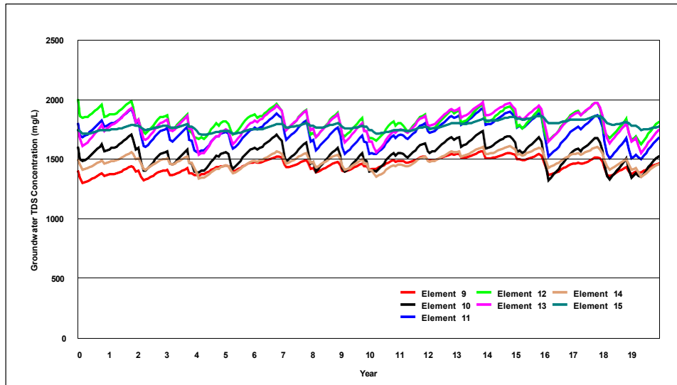
Figure 6-8 Simulated Groundwater TDS Concentrations – San Juan Creek Arm
